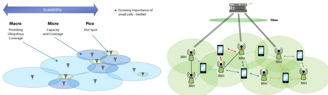
Figure 4: Changes to the wireless cell concept
