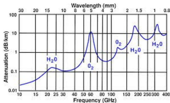
Figure 6: Atmospheric attenuation under different frequency bands, not including rain or clouds
